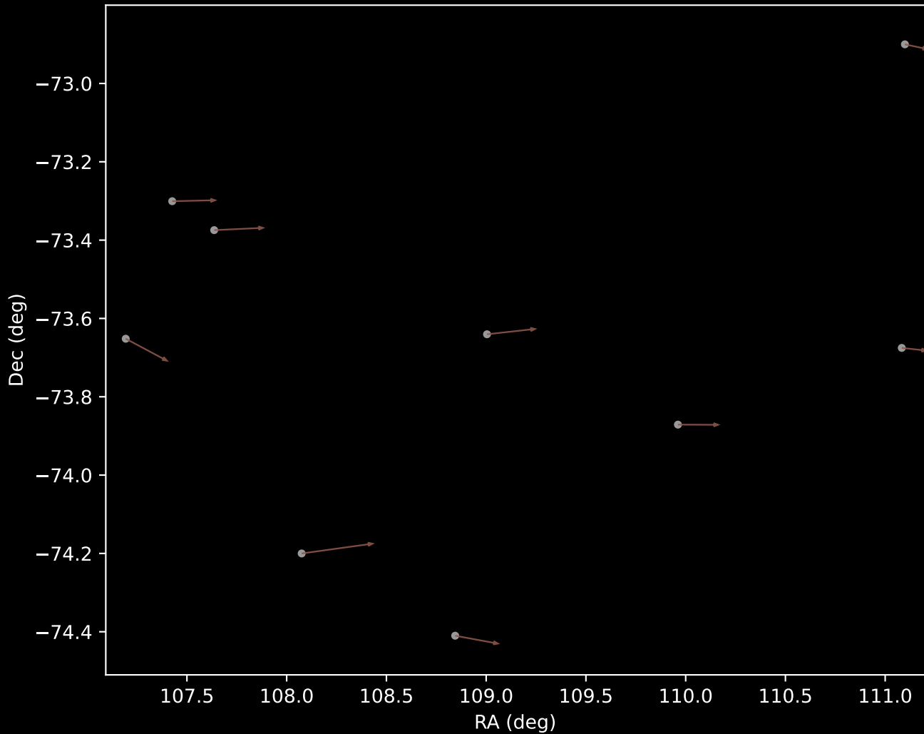
GALAH DR4 Cluster 10 Proper Motion Vectors (n=9)
