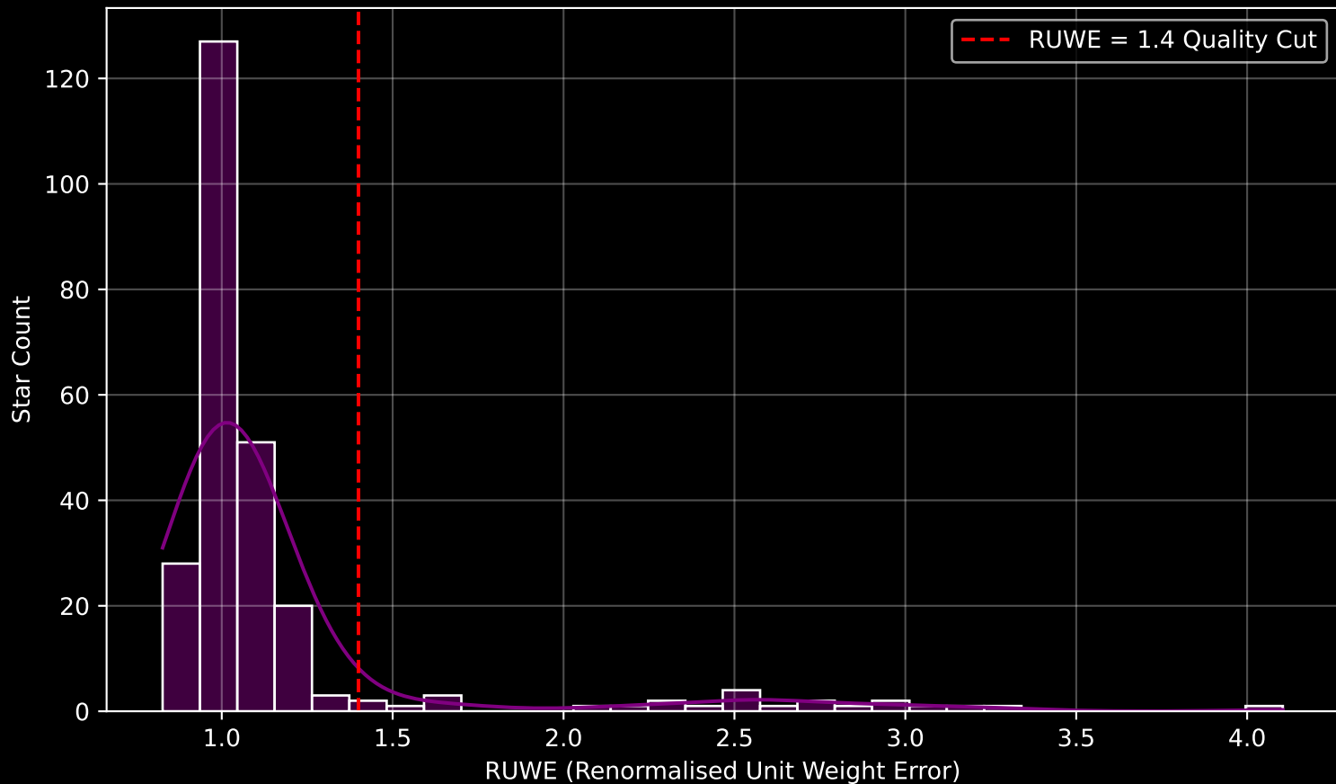
GALAH DR4 Field [88] RUWE Distribution (n= 254)
