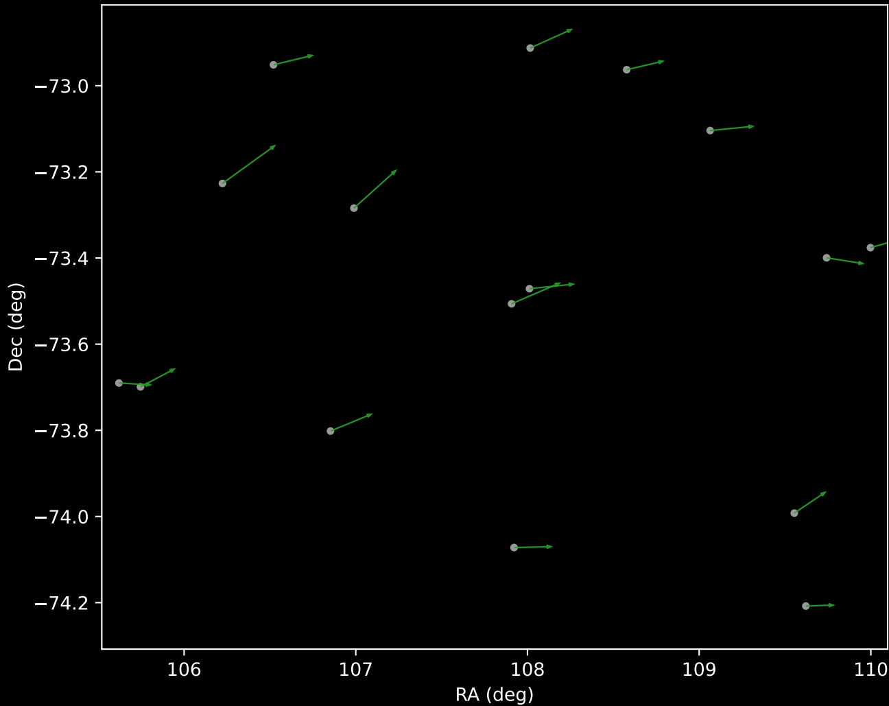
GALAH DR4 Cluster 4 Proper Motion Vectors (n=16)
