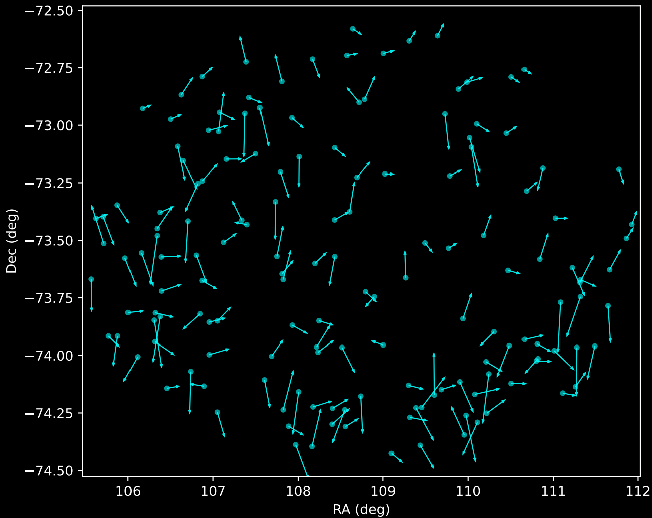
GALAH DR4 Noise Stream Proper Motion Vectors (n=153)
