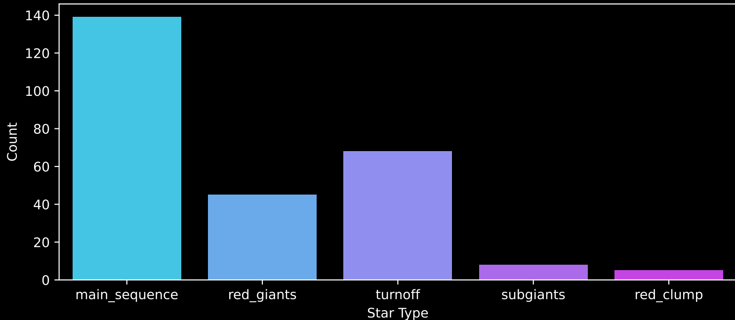
GALAH DR4 Field: [88] Count plot of Star Type
