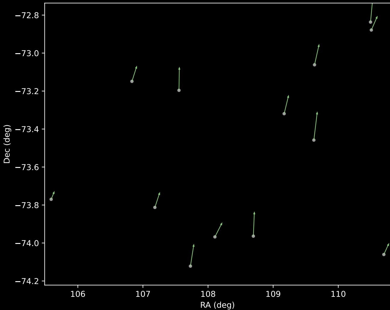
GALAH DR4 Cluster 5 Proper Motion Vectors (n=13)
